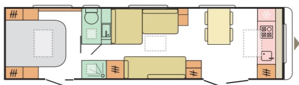
DAY LAYOUT
